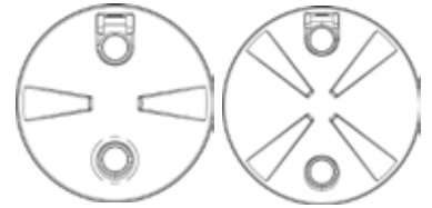
View of tank configuration. Left: 7,500L - 10,000L Right: 10,200L - 15,000L
