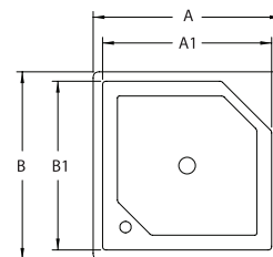
Cast Iron Access Cover & Frame # UG3083
